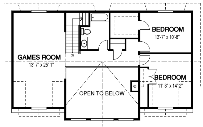
Upper Floor
